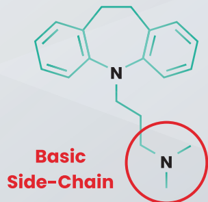
Tricyclic Antidepressants
